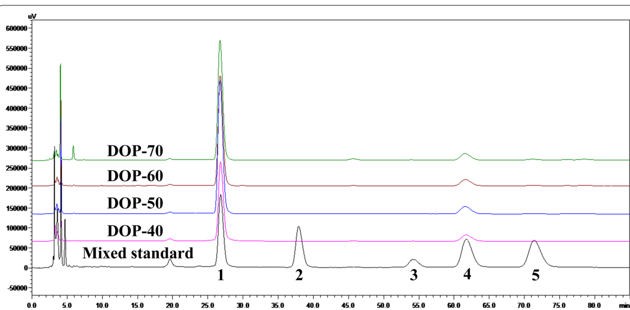
Fig. 4 HPLC profile of mixed monosaccharide standards (1-mannose, 2-rhamnose, 3-galactose, 4-glucose, and 5-arabinose), DOP-40, DOP-50, DOP-60, and DOP-70
