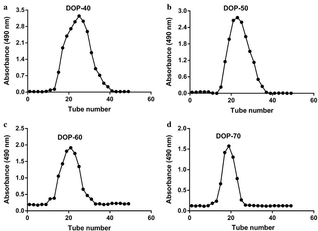
Fig. 3 Distilled NaCl elution curves of DOP-40 (a), DOP-50 (b), DOP-60 (c), and DOP-70 (d)
