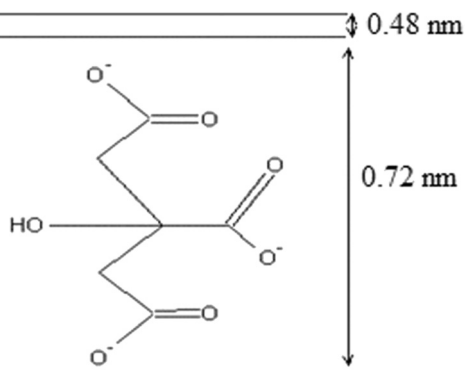
Fig. 2 Interlayer arrangement of citrate ion within the layers of Mg-Al LDH. The inter-layer arrangement was derived based on the basal spacing observed for the citrate LDH (1.20 nm) and the theoretical molecular size of citrate ion (0.72 nm)
