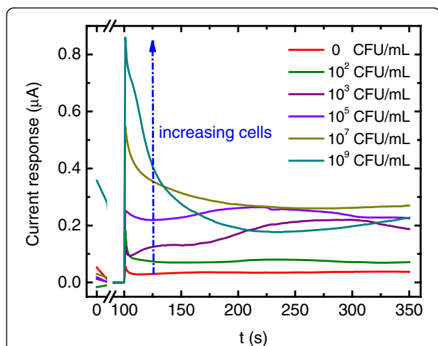
Figure 5 Chronoamperograms at the MAb-DW electrode with 10 µg/mL MAb at the working potential of 100 V vs. Ag/AgCl in citrate phosphate buffer (0.05 M, pH 5.5) solution with various cell concentrations (0 to 10 9 CFU/mL).
