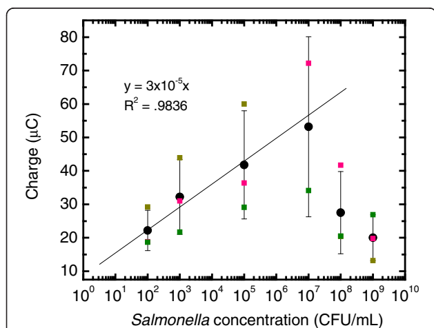
Figure 6 A plot of Salmonella typhimurium cell (CFU/mL) vs. the subtracted charge (µC) obtained at the MAb-DW electrode.
